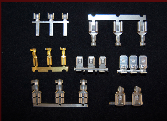
Uninsulated Quick Connects
