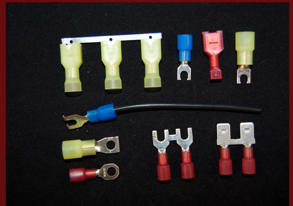
Partially and Fully Insulated Quick Connects
